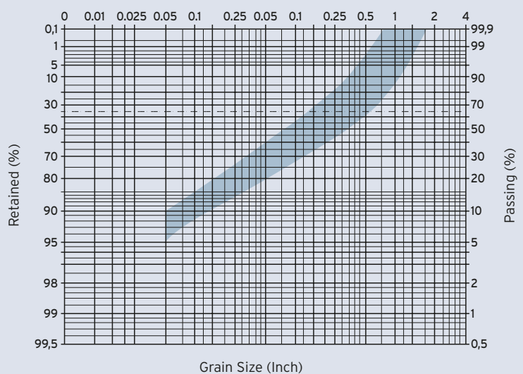
Granulation Curve HTI
